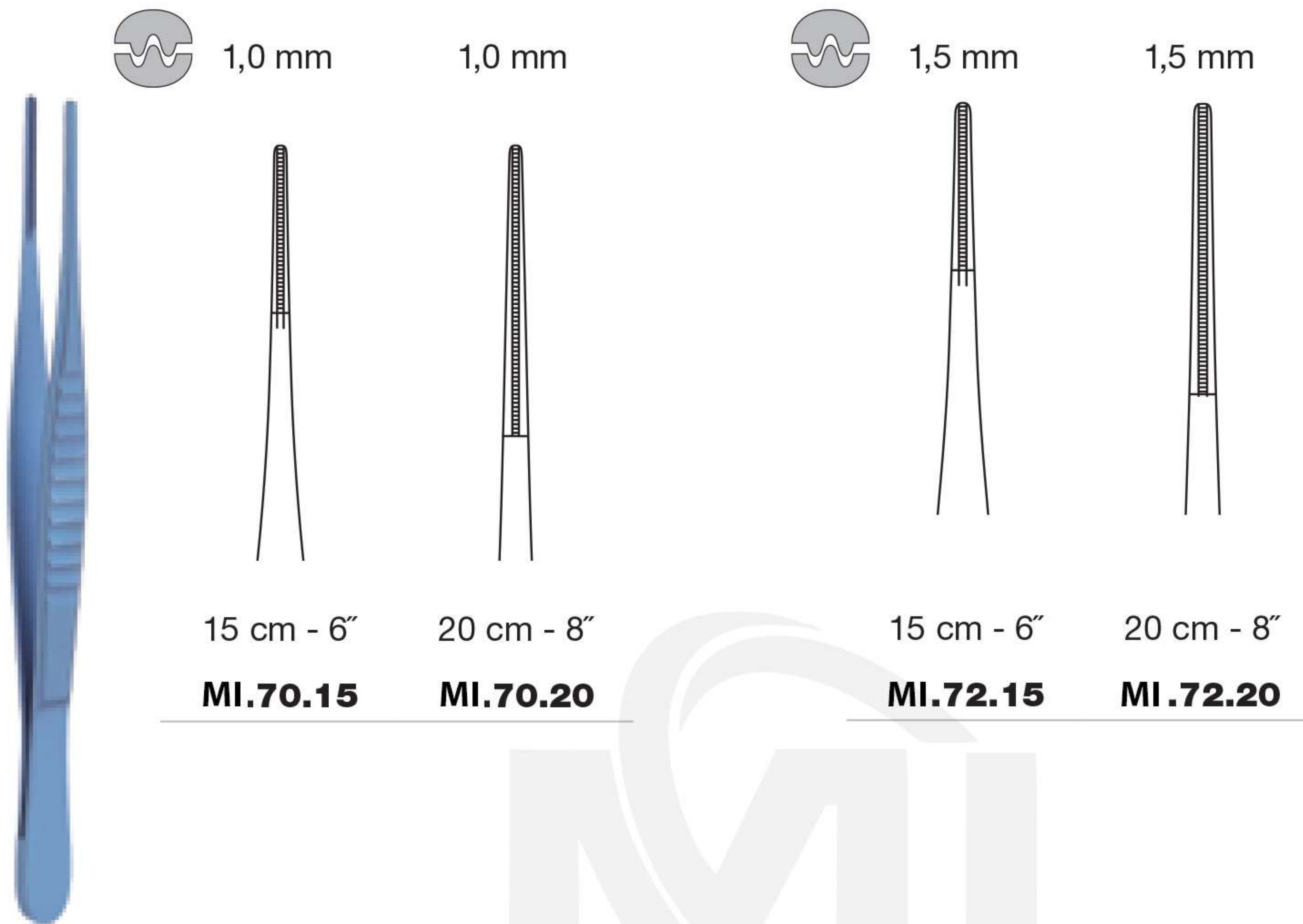
DeBakey "AT"
